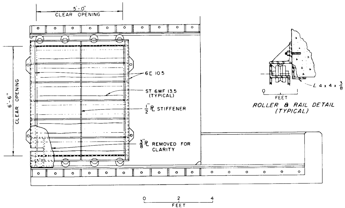
Fig. 4—Exterior elevation of blast door.
